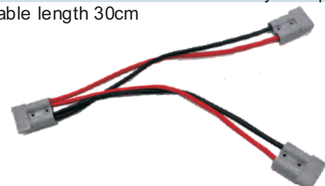
SF50592 50A connector leads with double connectors
