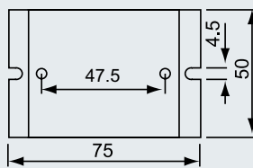
CSR-A01 (For CSR10A-40A)
