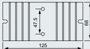
CSR-A02 (For CSR60A-100A)
