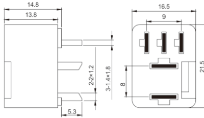
Terminal Layout(Bottom View)
