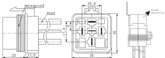
Terminal Layout(Bottom View)
