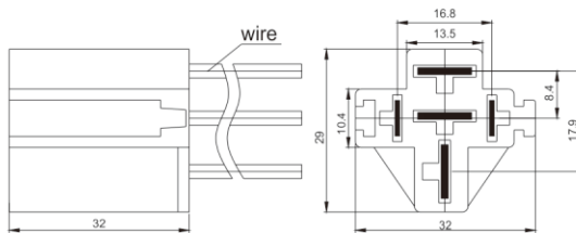
Terminal Layout(Bottom View)
