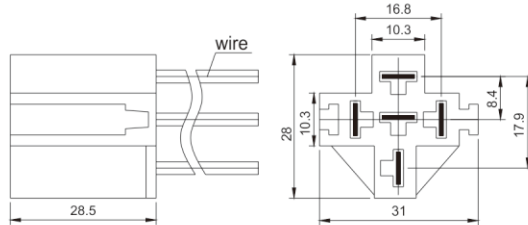
Terminal Layout(Bottom View)
