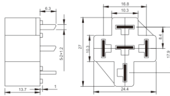
Terminal Layout(Bottom View)
