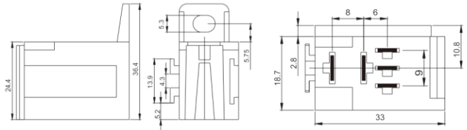
Terminal Layout(Bottom View)
