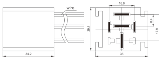
Terminal Layout(Bottom View)
