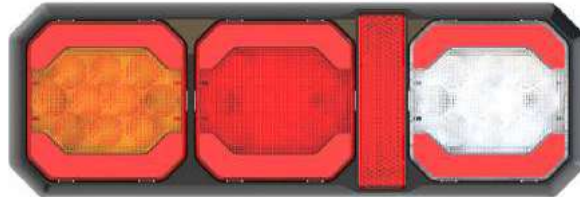
Z-T29F RPL - Rear Position Lamp / DI - Dynamic Direction Lamp / ST - Stop Brake / Reverse - Reversing Lamp / Reflex - Reflex Reflector
