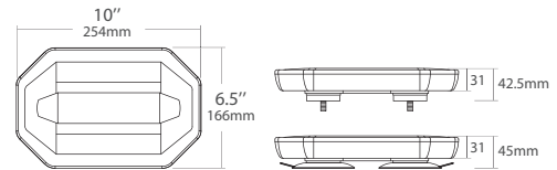
Z-W26S - Screw mount
