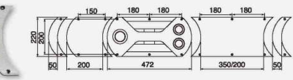
C 过渡板 Transition Board Dimension: 350/200 × 220
