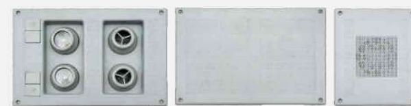
CD26-009 带灯出风口 过渡板 Wind outlet of reading lamp/Transition plate 外形尺寸(Dimension): 330 × 220 喇叭罩(Horn cover Dimension): 185 × 220 过渡板尺寸(Transition plate Dimension): 330 × 220
