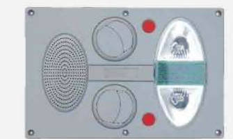
CD25-028 带灯出风口 Wind outlet of reading lamp 外形尺寸(Dimension): 330 × 220 开孔尺寸(Dimension): 295 × 200
