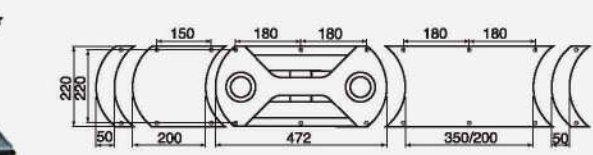
C 过渡板 Transition Board Dimension: 350/200 × 220
