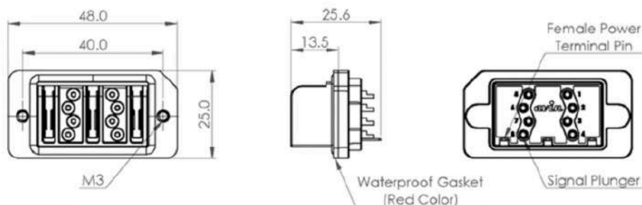
Female Connector
