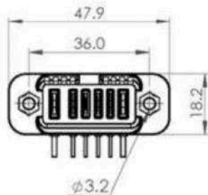
Female Connector
