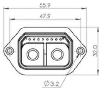
Female Connector
