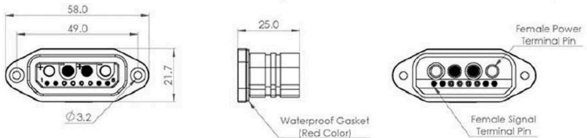
Female Connector
