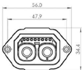
Female Connector
