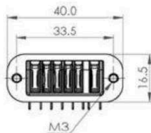
Female Connector
