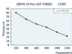
■ 电机特性曲线 Motors Performance Curves
