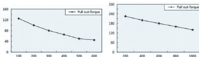
■ 电机特性曲线 Motors Performance Curves
