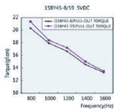
电机特性曲线 Motors Performance Curves
