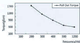
电机特性曲线 Motors Performance Curves
