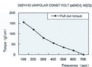
■ 扭矩曲线图 Torque Characteristics
